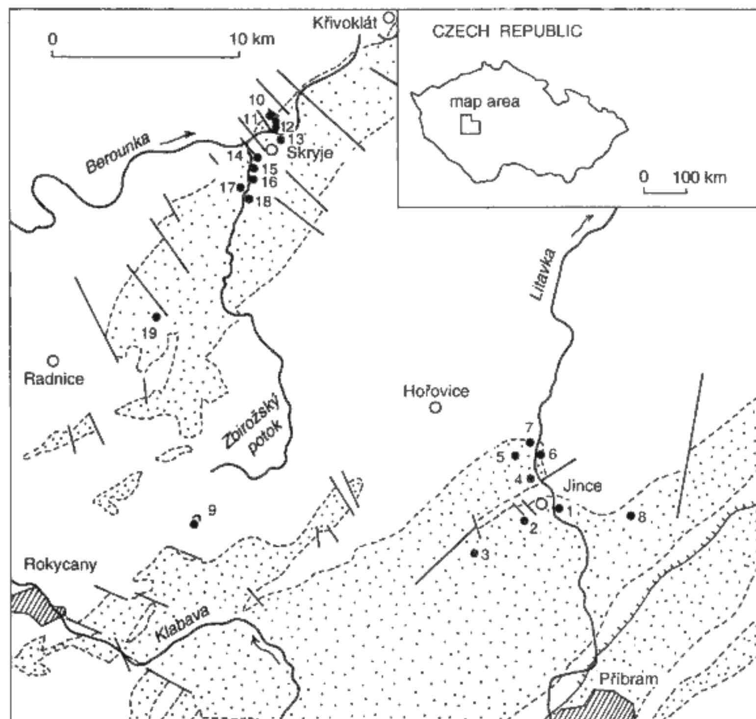
1. Sketch map of the Central Bohemian Cambrian showing the position of the localities. 1 - Vinice; 2 - Vystrkov; 3 - Koníčec; 4 - Jince - Ovčín; 5 - Felbabka - Potůček; 6 - Rejkovice; 7 - Ostrý; 8 - Písky; 9 - Medový Újezd; 10 - Kamenná hůrka; 11 - Pod tmím; 12 - Mouth of the Karáskova rokle Gorge; 13 - Luh; 14 - Slapnice - camp; 15 - Dlouhá hora; 16 - Dubinky; 17 - Jezírka; 18 - Buchava; 19 - Biskoupky. Dotted area corresponds to the present occurrence of the Cambrian rocks, including the Lower Cambrian conglomerates and sandstones and the Upper Cambrian volcanites.
