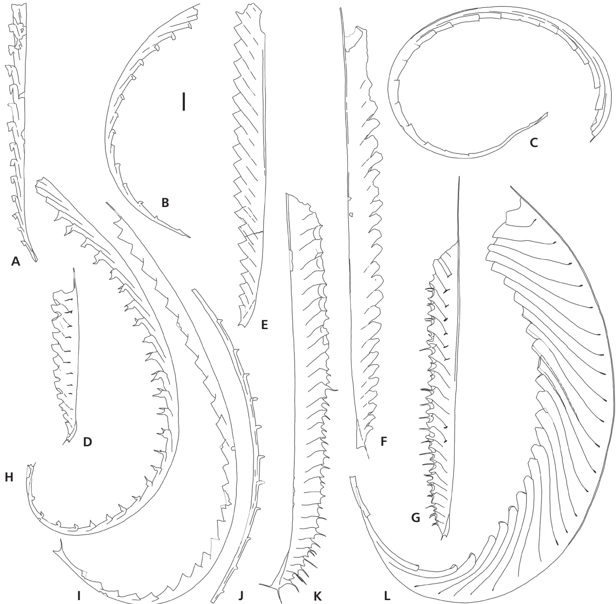
Figure 23. Age-diagnostic Ludfordian graptolites. • A – Slovinograptus balticus (Teller), PŠ 2018, latilobus–balticus Biozone. • B – Neocullograptus inexpectatus (Bouček), PŠ 2100, inexpectatus Biozone. • C – Egregiograptus rinellae Koren' & Sujarkova, PŠ3060, tenuis Biozone. • D – Pseudomonoclimacis dalejensis (Bouček), PŠ 3049, tenuis Biozone. • E – Pristiograptus fragmentalis (Bouček), PŠ 2309, fragmentalis Biozone. • F – Pseudomonoclimacis latilobus (Tsegelnyuk), PŠ 2006, latilobus–balticus Biozone. • G – Saetograptus leintwardinensis (Lapworth), PŠ 3252, leintwardinensis Biozone. • H – Neocullograptus kozlowskii Urbanek, PŠ 670/1, kozlowskii Biozone. • I – Bohemograptus tenuis (Bouček), PŠ 3134, tenuis Biozone. • J – Crinitograptus? sp., PŠ 2308, latilobus–balticus Biozone. • K – Saetograptus clavulus (Perner), PŠ 3174, upper leintwardinensis Biozone. • L – Polonograptus podoliensis , PŠ 620/1, kozlowskii Biozone. A–G, I–K – Všerádice-trench; H, L – Kosov quarry, 3 rd level. All figures \times 5 , scale bar represents 1 mm.
