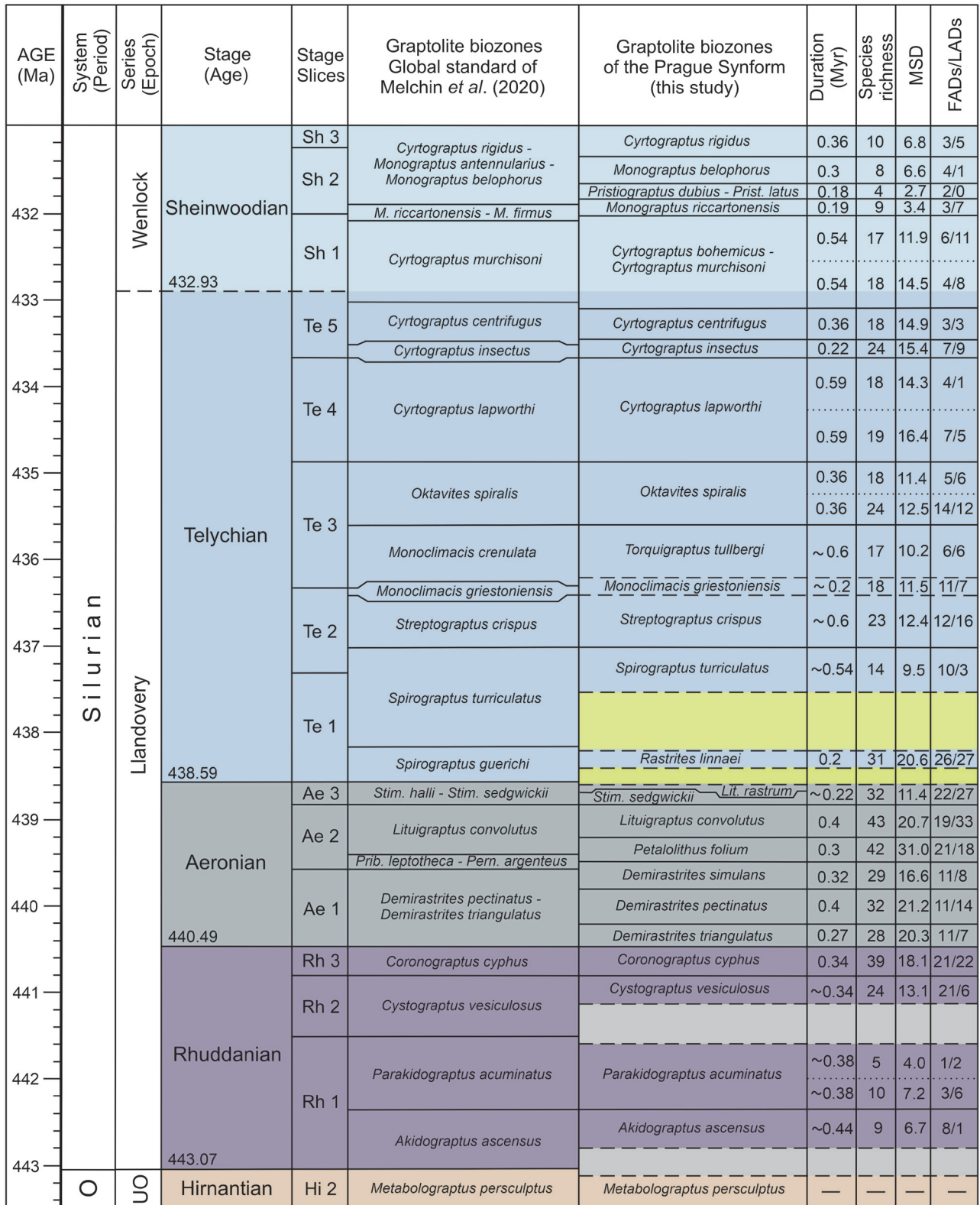
Figure 7. Silurian time scale, geochronology, chronostratigraphy and graptolite biostratigraphy. Time duration of graptolite biozones recognized in the Prague Synform is derived from correlation with the standard graptolite biozonal scheme calibrated with the Silurian time scale (Melchin et al. 2020) and stage slices of Cramer et al. (2011). Dashed horizontal lines mark tentative delineation of zonal boundaries. Dotted horizontal lines indicate subdivision or particularly long biozones into two or three subintervals of equal duration. Diversity trends are documented by species richness per biozone, mean standing diversity (MSD), and originations/extinctions ratio (FADs/LADs). Basin-wide gaps in the Rhuddanian stratigraphical record
