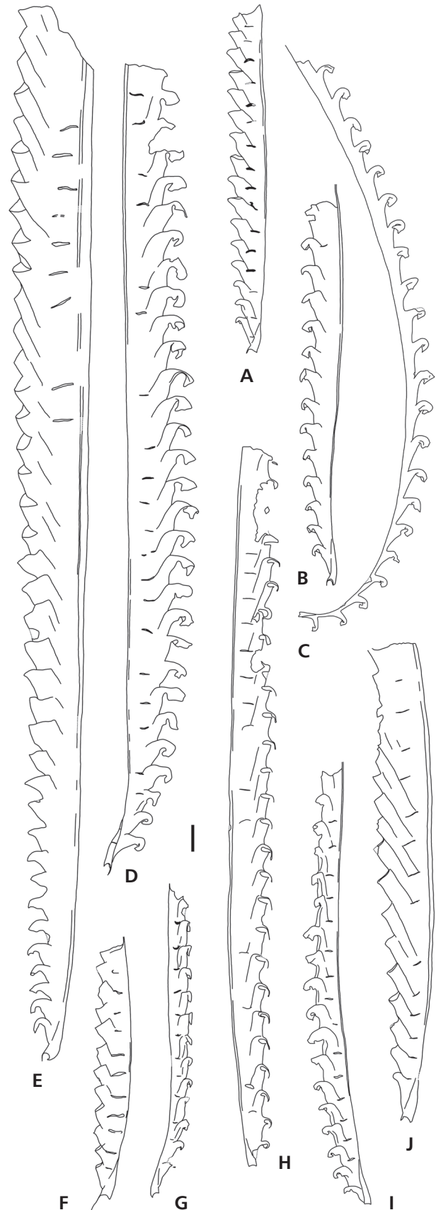
Figure 25. Age-diagnostic graptolites of the Přidolí Series. • A – Skalograptus ultimus (Perner), PŠ 4364, parultimus – ultimus Biozone. • B – Wolynograptus? hornyi (Jaeger), HJ059, lochkovens Biozone. • C – Formosograptus formosus (Bouček), PŠ 4368, parultimus – ultimus Biozone. • D – Wolynograptus bouceki (Přibyl), PŠ 4365, bouceki Biozone. • E – Skalograptus lochkovens (Přibyl), PŠ 4477, lower bouceki Biozone. • F – Skalograptus parultimus (Jaeger), PŠ 4418, lower lochkovens Biozone. • G – Slovinograptus beatus (Koren'), PŠ 4411, upper bouceki Biozone. • H – Uncinatograptus pridoliensis (Přibyl), L62904a, lochkovens Biozone. • I – Wolynograptus perneri (Bouček), BB 6995, perneri Biozone. • J – Skalograptus transgrediens (Perner), PŠ 4402, upper bouceki Biozone. A–C – Kosov quarry, 1 st level; D–G, J – Radotín-Hvižd'alka; H – Lochkov-Marble Quarry; J – Praha-Podolí, quarry. All figures × 5, scale bar represents 1 mm.
